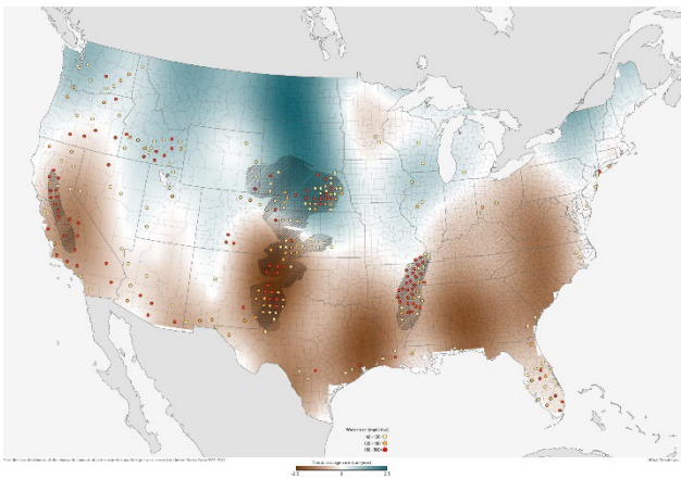
Figure 3. Map of the change in annual water storage per year across the United States from 2003-2012, as estimates from the GRACE satellite. Storage increases are in shades of blue, while storage decreases are in shades of brown. The dots indicate counties where water use exceeded 60 million of gallons per day or more as of 2005, according to data from the U.S. Geological Survey.
